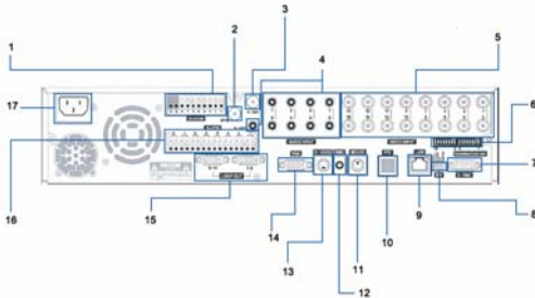
Back Panel
